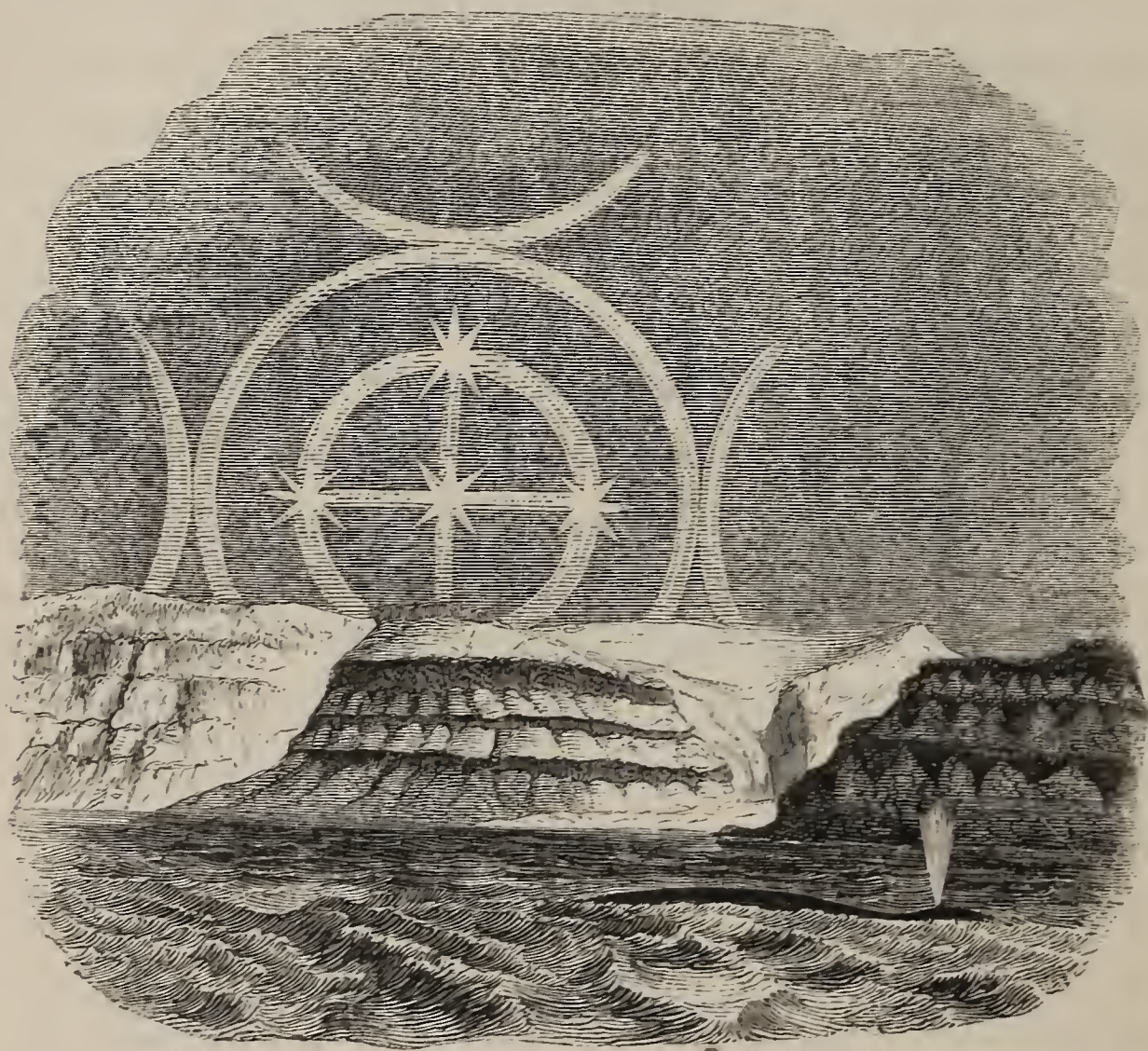
MOCK SUNS.
